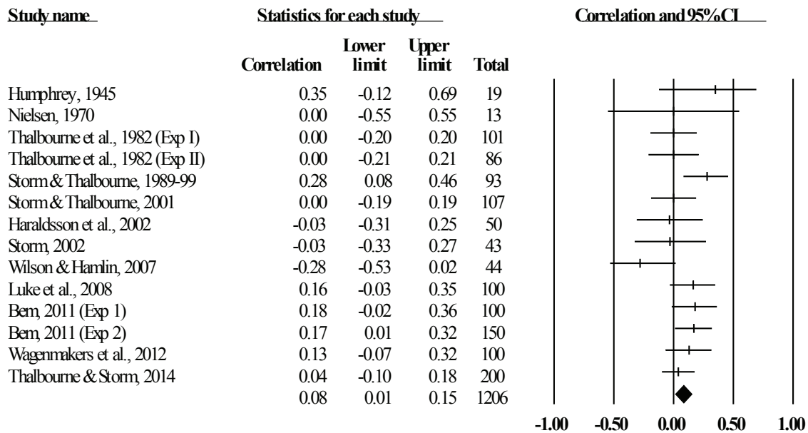
Figure 4. Meta-analysis of the relationship between extraversion and psi performance in forced-choice precognition experiments.
