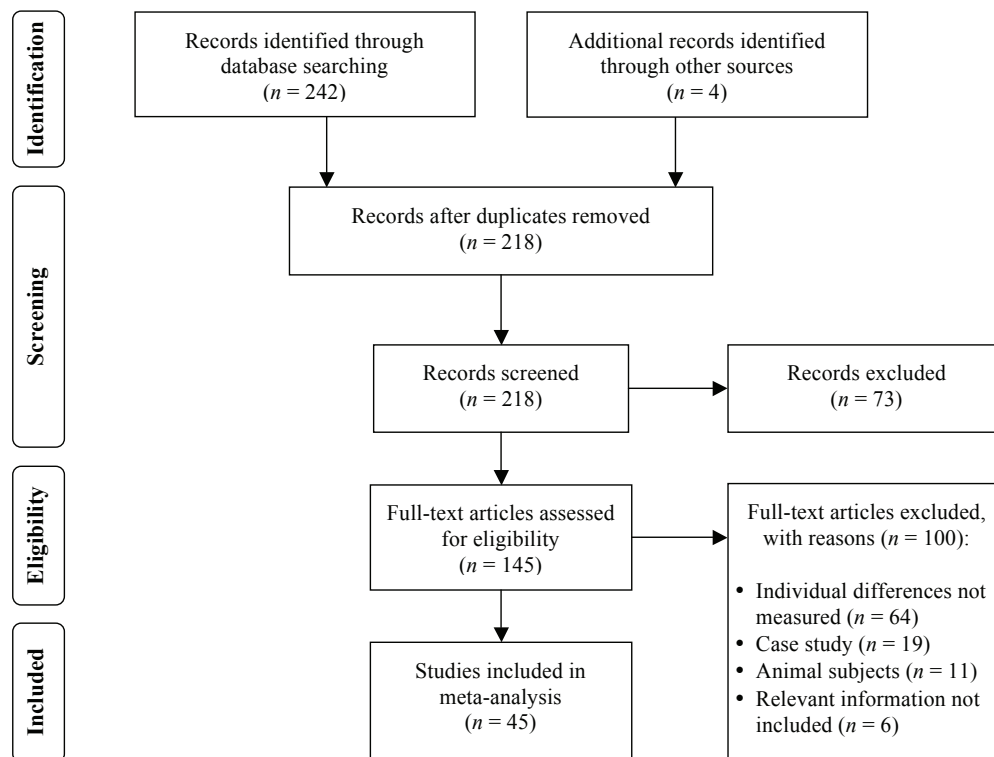
Figure 1. A flow diagram illustrating the database search and screening stages involved in this meta-analysis. 2
